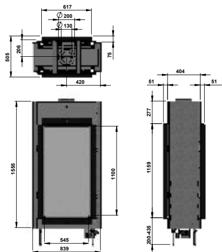
Trimline 55XHTunnel
